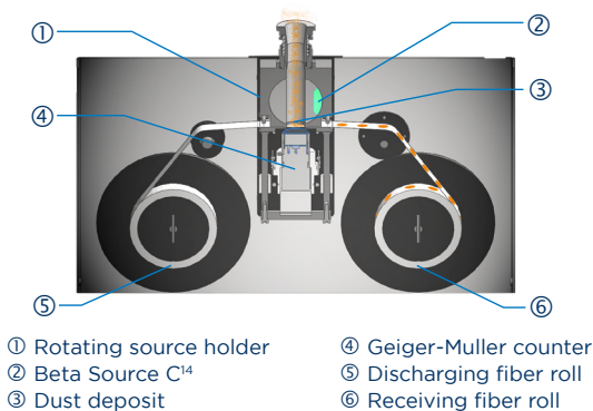
MP101M - operating principle
